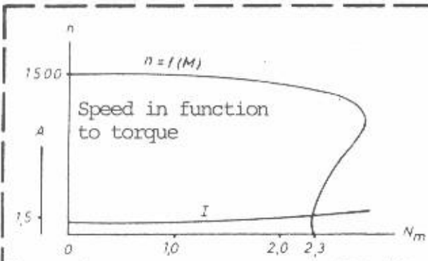
Three-phase cage rotor motor 004.003
