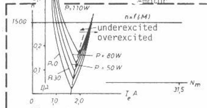
Three-phase synchronous generator 004.021
