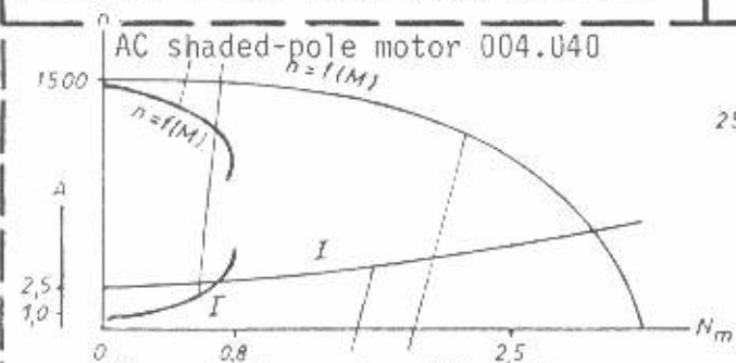
AC shaded-pole motor 004.040
