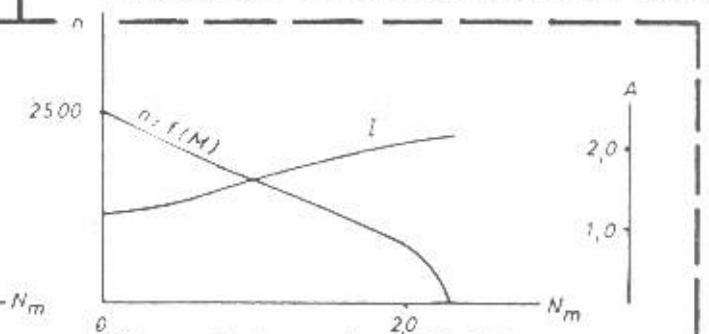
AC repulsion motor 004.031
