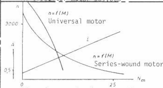
DC series-wound universal motor 004.001
