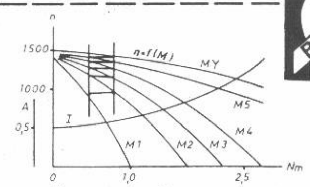
Three-phase slip ring rotor motor 004.004
