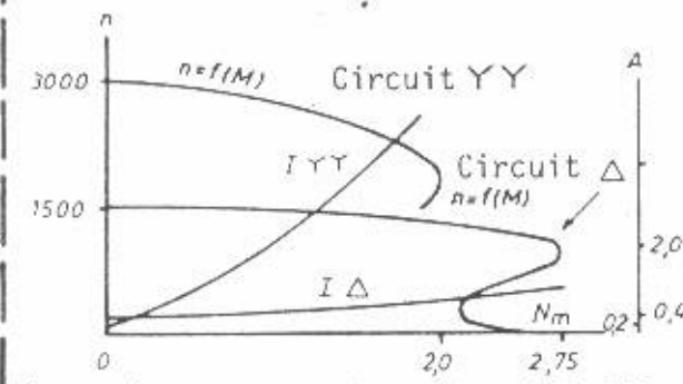
Three-phase cage rotor motor 004.029a
